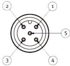
connector view 5 pin M 12×1 RSFM5
